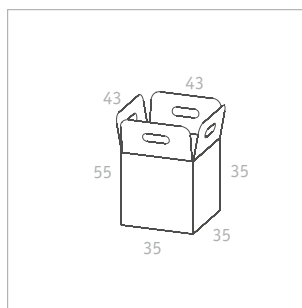
Box 40 Volume planter 26 l Planting depth 25 cm Weight 13 kg [15 kg]
