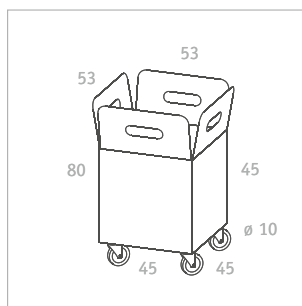
Box 65 Volume planter 26 l Planting depth 39 cm Weight 22 kg [25 kg]
